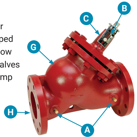
Flanged / grooved 4" – 12"
