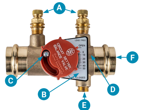
Circuit Setter Plus Lead-Free* Brass 1/2" – 3"
