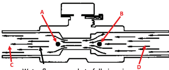
Water flow expands to full pipe size, water velocity is decreased and static pressure is "recovered".
