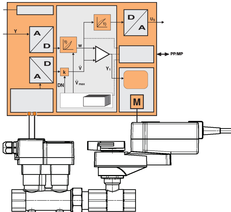
Block diagram
