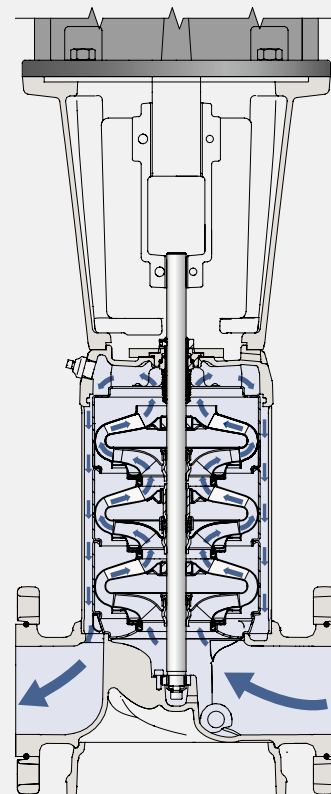
In-line multi-stage centrifugal pump
