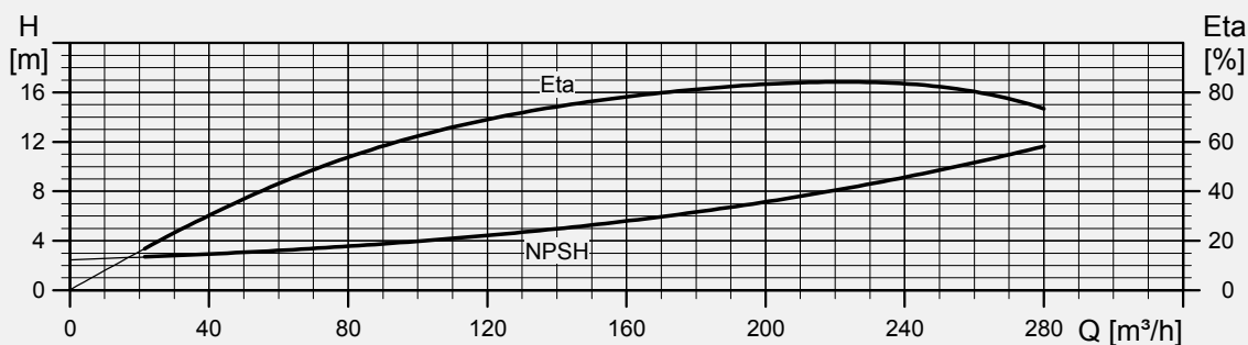
Efficiency and NPSH curves for the Grundfos submersible pump type 1100S. The pump's nameplate typically notes the pump's flow at best efficiency. Another number typically refers to the number of bowls and thereby how much pressure the pump can produce.
