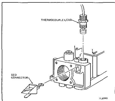
Fig. 1—Install ECO connector into gas control at thermocouple terminal location.
