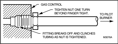
Fig. 4—Always use new compression fitting.
