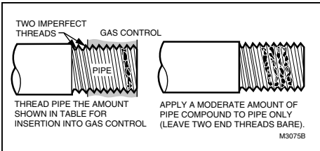
Fig. 2—Use moderate amount of pipe compound.
