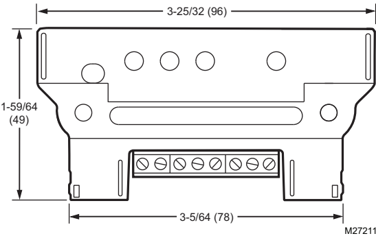
Fig. 1. Q7130,Q7230,Q7330 Modutrol IV Interface Module dimensions in in. (mm).
