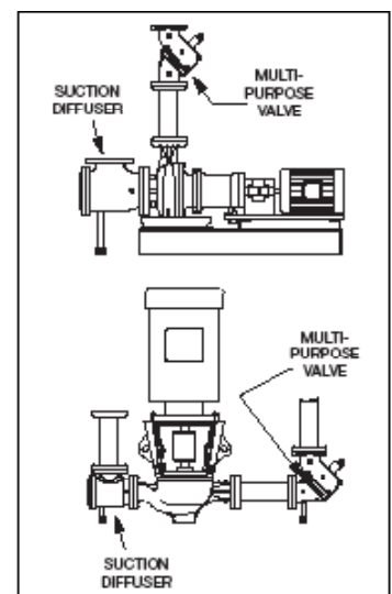
FIGURE 1: PIPING DIAGRAM
